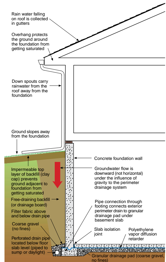
Figure 9 Below grade groundwater management
