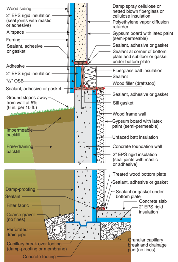
Figure 14 Additional interior basement insulation
