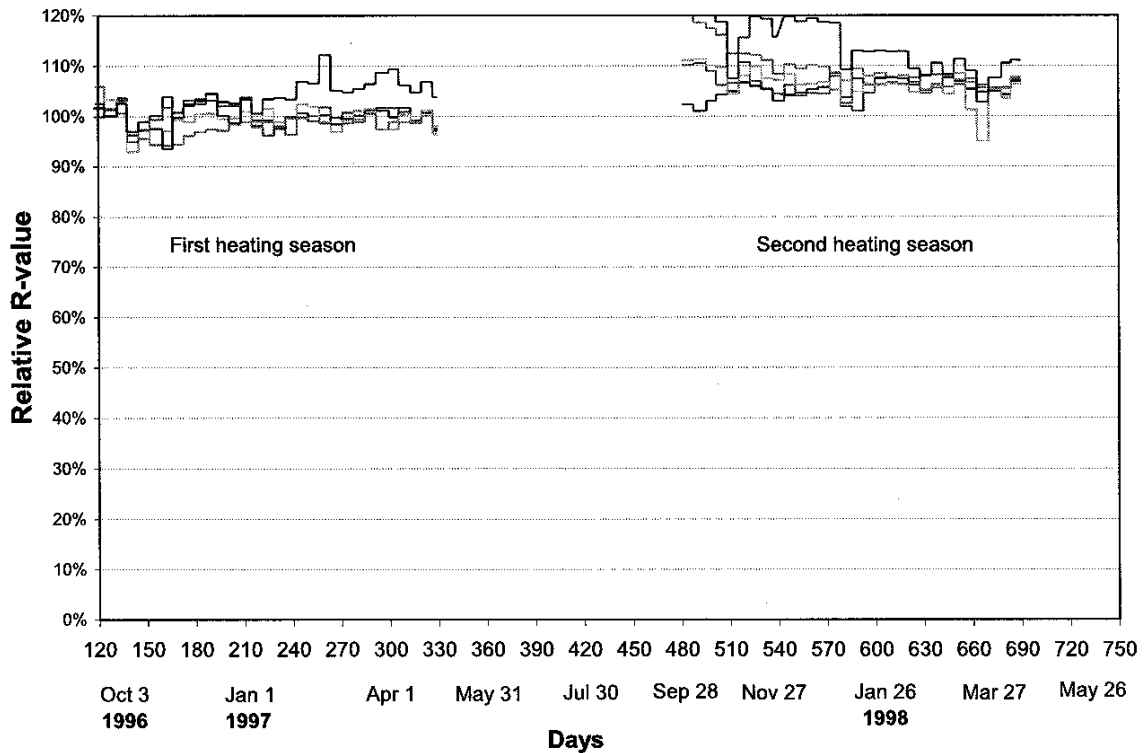
Figure 2 Range of Thermal Performance Result for Specimens on One Test Wall (EPS Type 1, EPS Type 2, Glass Fibre, Mineral Fibre and Sprayed-in-Place Polyurethane Foam)
