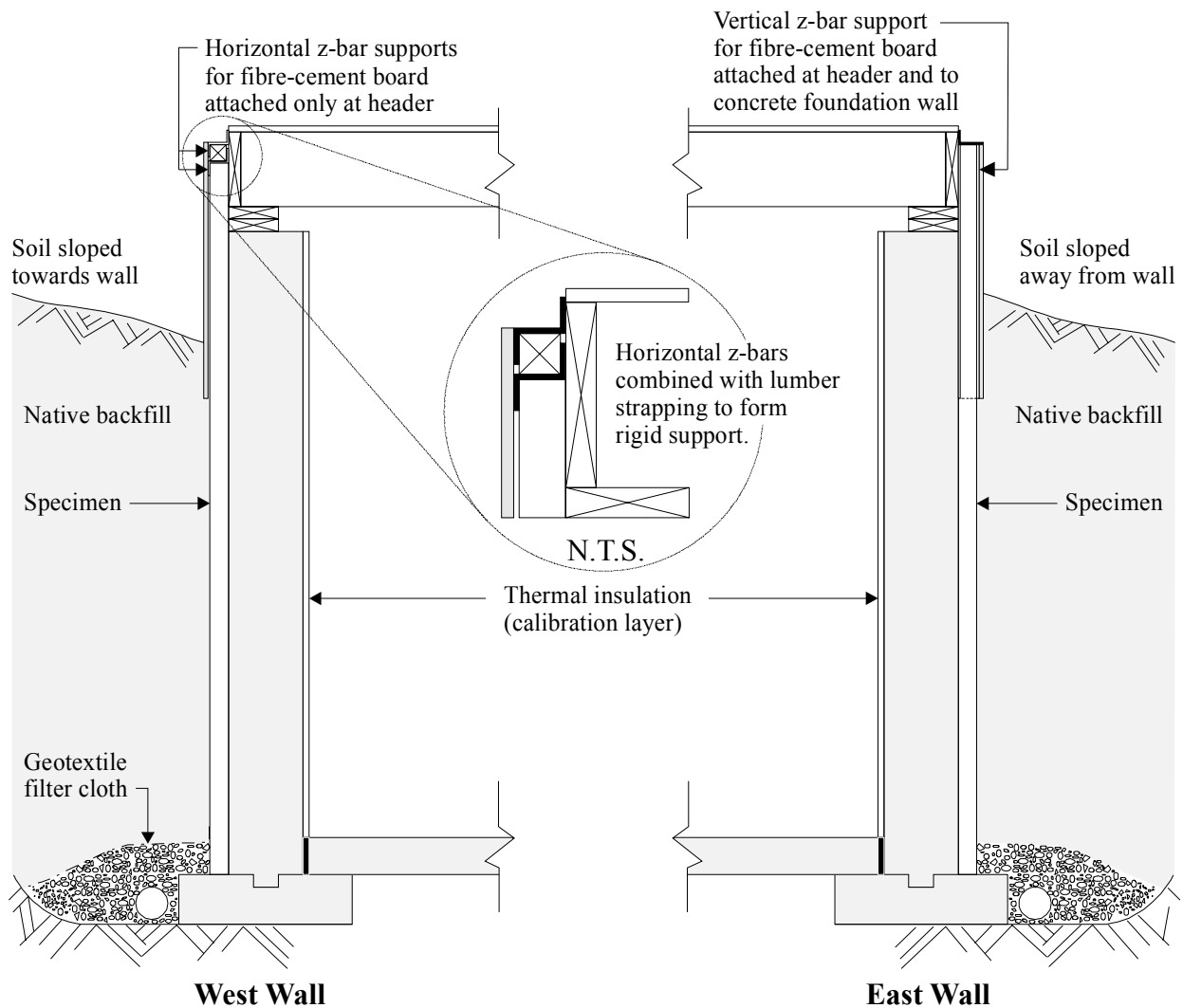
Figure 1 Wall Sections Used in EIBS Field Testing
