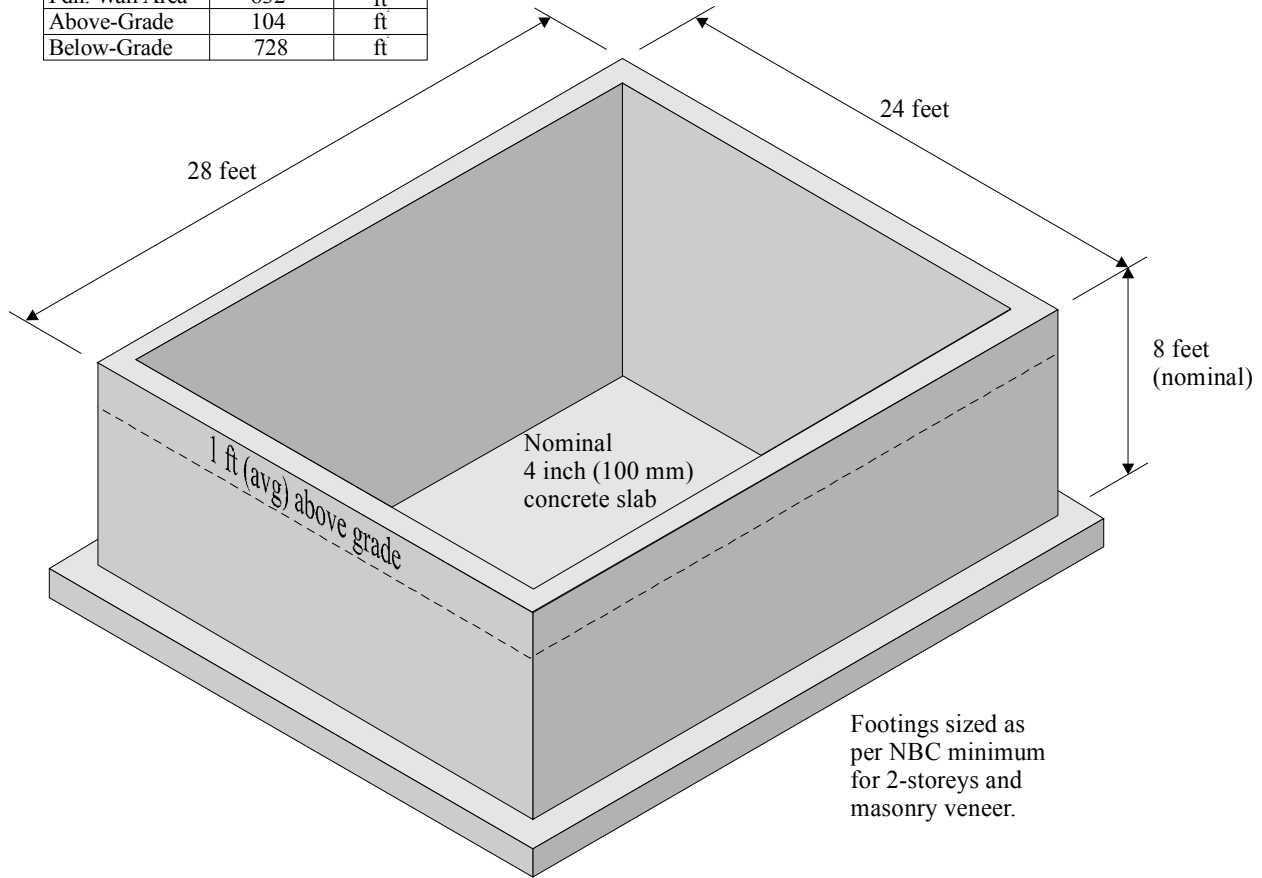
Figure 3 Base Case Basement Model Used in Economic Assessment Study
